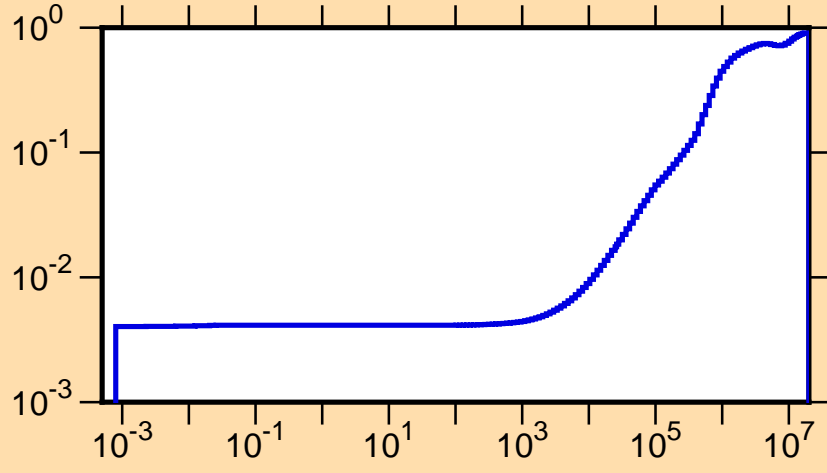
\mu vs. E for ^{167}\text{Yb}(\text{mt251})
