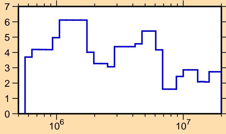
\Delta\sigma/\sigma vs. E for ^{167}\text{Yb}(n, \text{el.})
