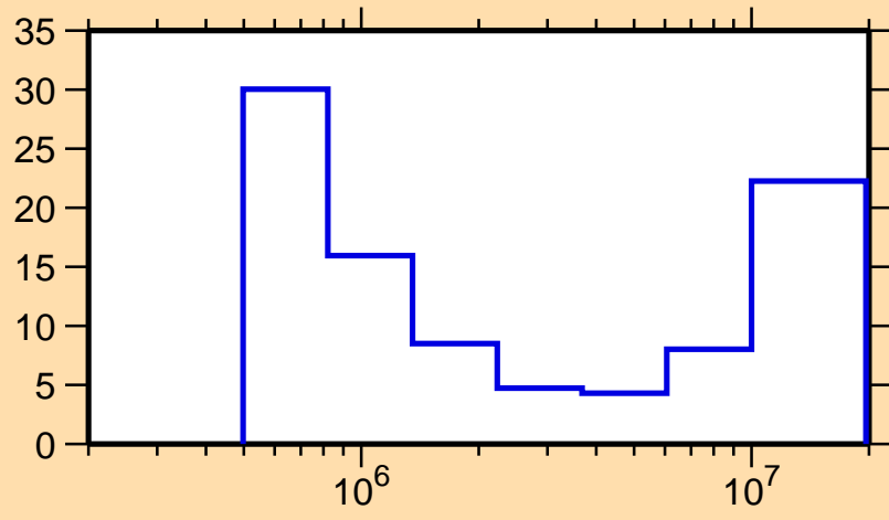
\Delta\sigma/\sigma vs. E for ^{167}\text{Yb}(n,n\text{cont.})
