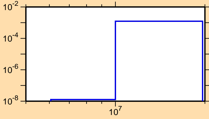
\sigma vs. E for ^{167}\text{Yb}(n,d)
