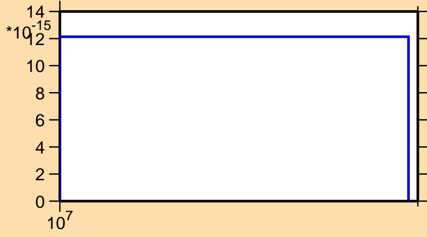
\sigma vs. E for ^{168}\text{Yb}(n,pd)
