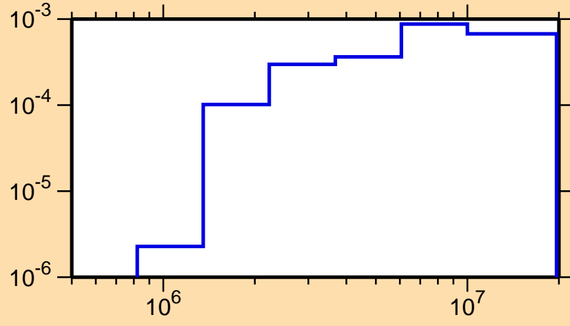
\sigma vs. E for ^{168}\text{Yb}(n,n_4)
