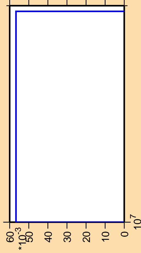
\Delta\sigma/\sigma vs. E for ^{168}\text{Yb}(n,pd)
