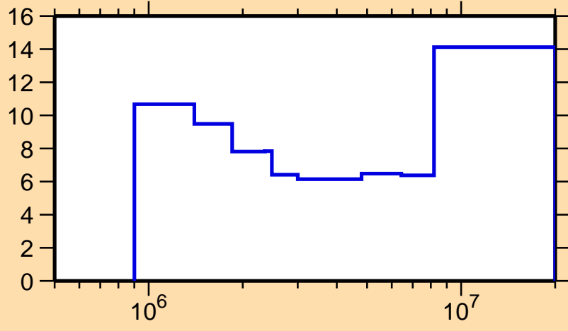
\Delta\sigma/\sigma vs. E for ^{168}\text{Yb}(n,\text{inel.})
