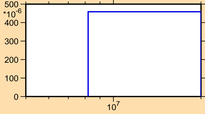
\sigma vs. E for ^{168}\text{Yb}(n,3n)
