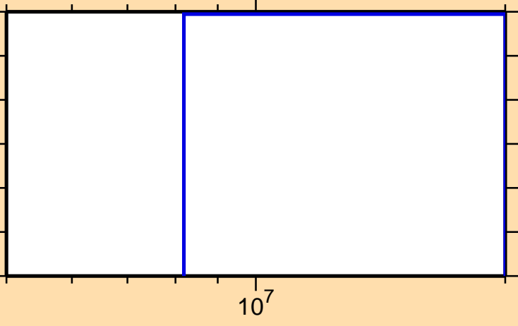
\sigma vs. E for ^{168}\text{Yb}(n,\text{pd})
