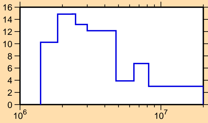
\Delta\sigma/\sigma vs. E for ^{168}\text{Yb}(n, el.)
