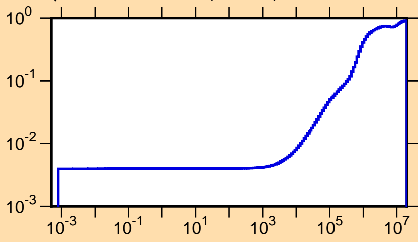
\mu vs. E for ^{169}\text{Yb}(\text{mt251})
