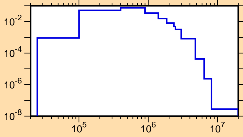
\sigma vs. E for ^{169}\text{Yb}(n,n_3)
