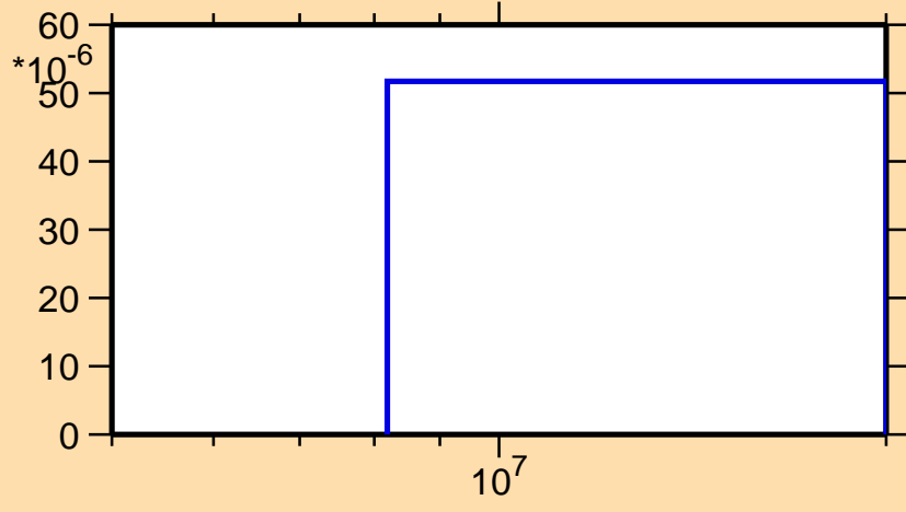
\sigma vs. E for ^{169}\text{Yb}(n,t)
