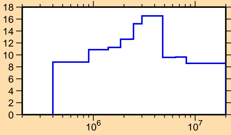
\Delta\sigma/\sigma vs. E for ^{169}\text{Yb}(n, el.)
