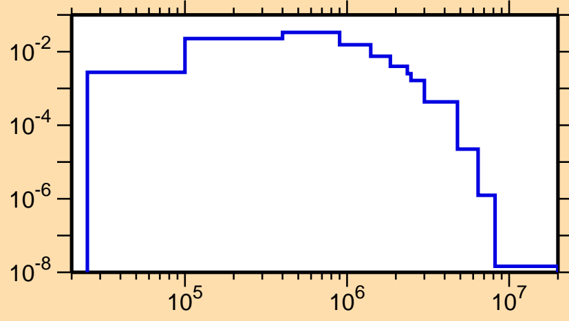
\sigma vs. E for ^{169}\text{Yb}(n,n_1)
