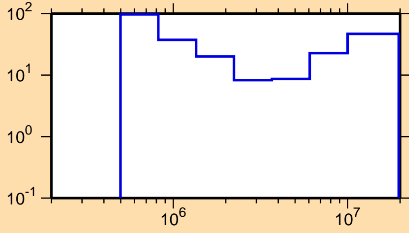
\Delta\sigma/\sigma vs. E for ^{169}\text{Yb}(n,n\text{cont.})
