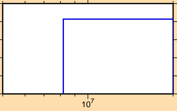
\sigma vs. E for ^{169}\text{Yb}(n,\text{pt})
