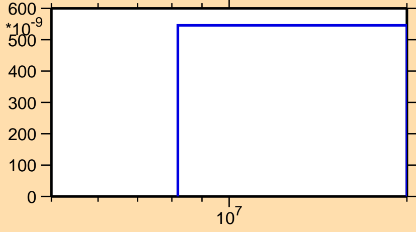
\sigma vs. E for ^{169}\text{Yb}(n,2n\alpha)
