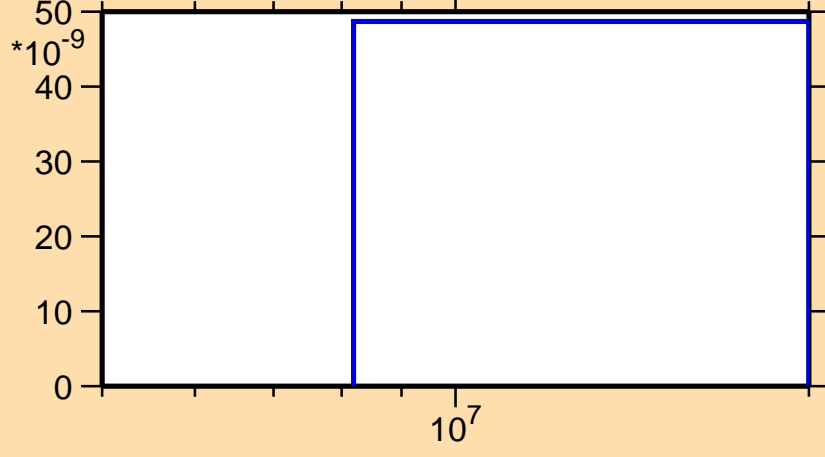
\sigma vs. E for ^{169}\text{Yb}(n,2np)
