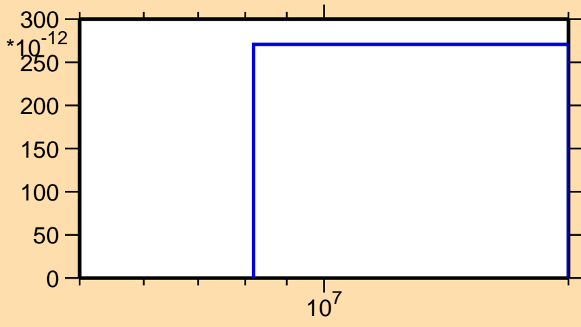
\sigma vs. E for ^{169}\text{Yb}(n,\text{He3})
