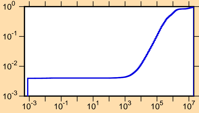
\mu vs. E for ^{171}\text{Yb}(\text{mt251})
