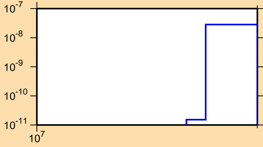
\sigma vs. E for ^{171}\text{Yb}(n,nt)
