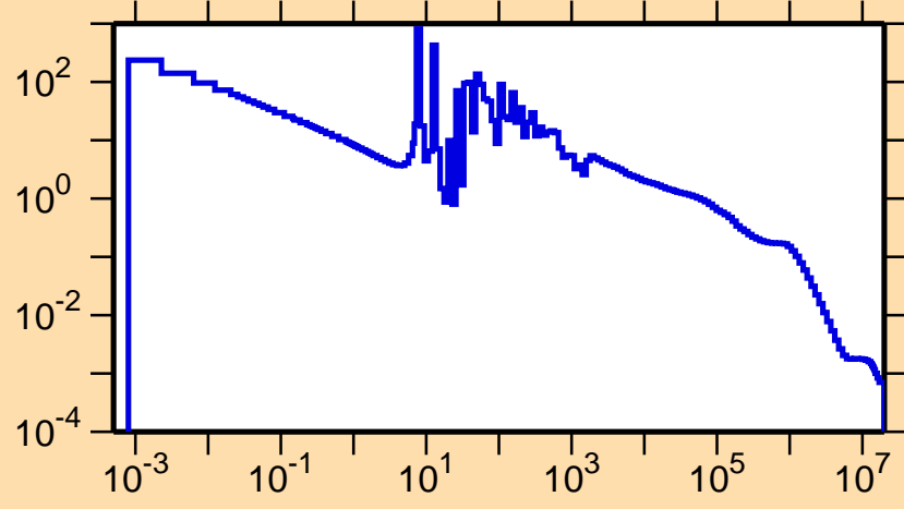
\sigma vs. E for ^{171}\text{Yb}(n,\gamma)
