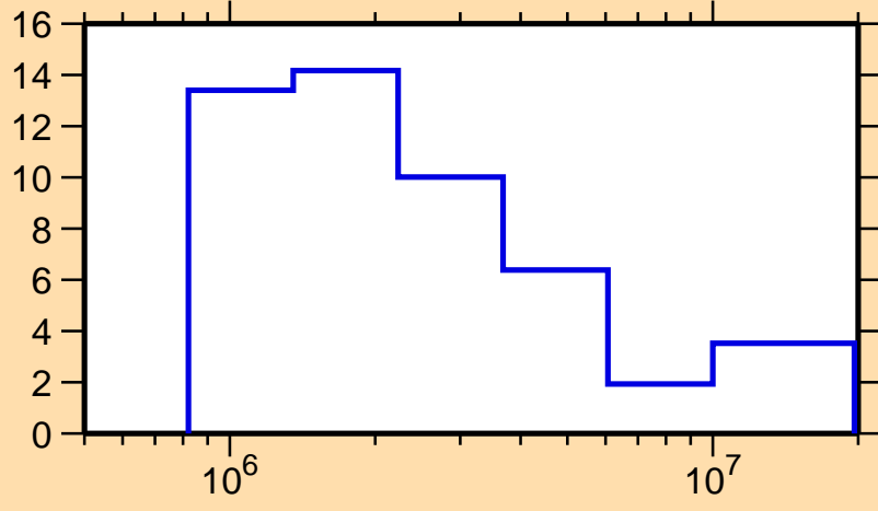
\Delta\sigma/\sigma vs. E for ^{171}\text{Yb}(n, tot.)
