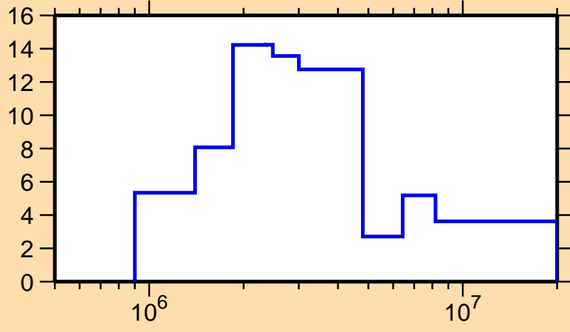
\Delta\sigma/\sigma vs. E for ^{171}\text{Yb}(n, el.)
