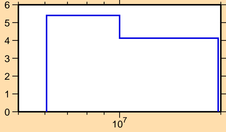
\Delta\sigma/\sigma vs. E for ^{172}\text{Yb}(n,2n)
