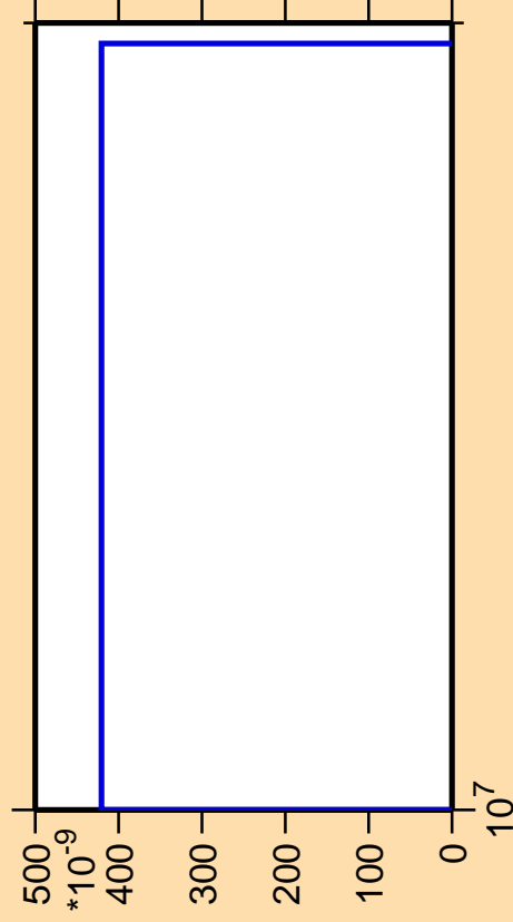
\Delta\sigma/\sigma vs. E for ^{172}\text{Yb} (mt 11)
