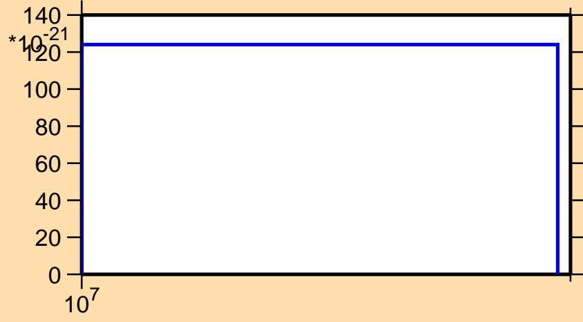
\sigma vs. E for ^{172}\text{Yb} (mt 11)
