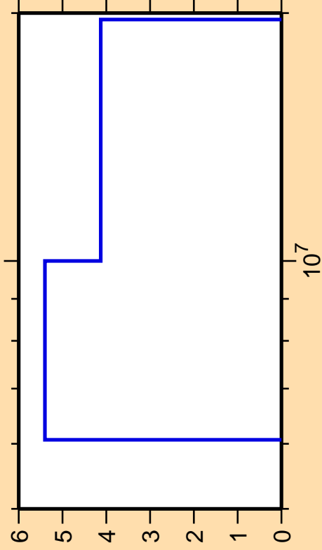
\Delta\sigma/\sigma vs. E for ^{172}\text{Yb}(n,2n)
