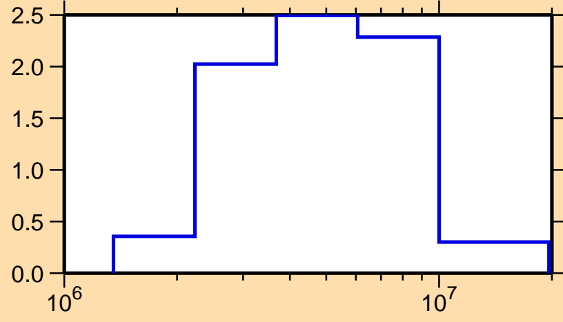
\sigma vs. E for ^{172}\text{Yb}(n,n\text{cont.})
