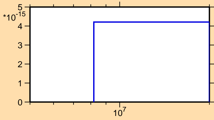
\sigma vs. E for ^{172}\text{Yb}(n,p\alpha)
