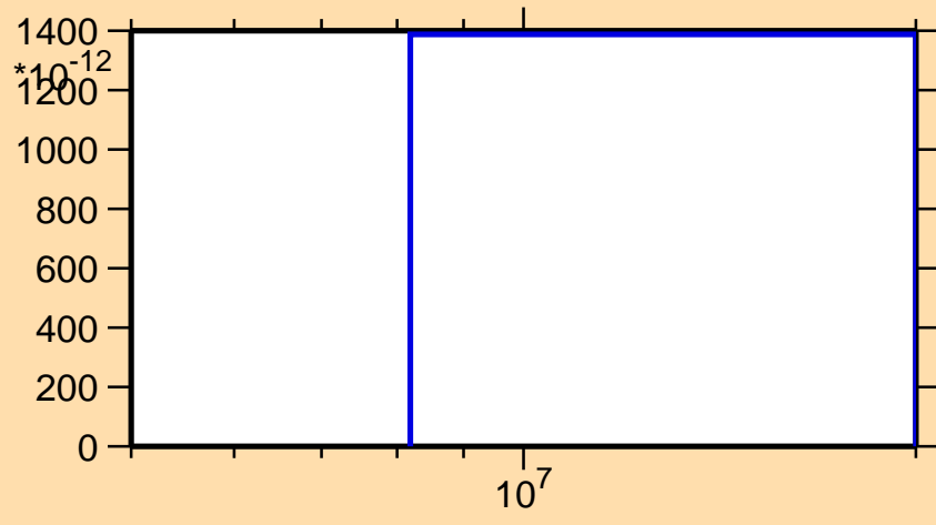
\sigma vs. E for ^{172}\text{Yb}(n,\text{nd})
