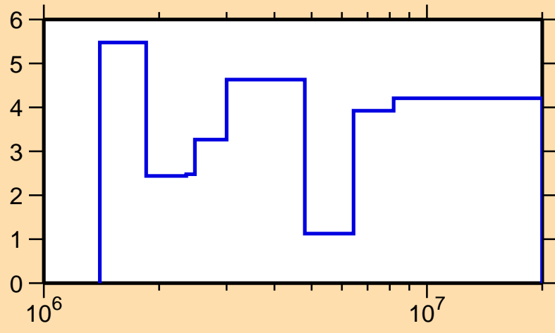
\Delta\sigma/\sigma vs. E for ^{172}\text{Yb}(n, el.)
