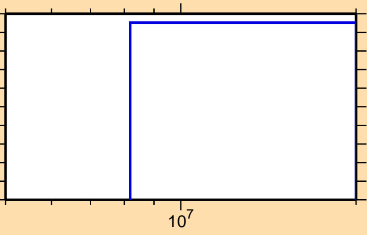
\sigma vs. E for ^{172}\text{Yb}(n,t)
