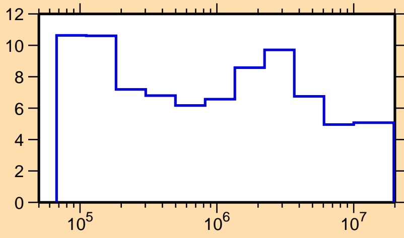
\Delta\sigma/\sigma vs. E for ^{173}\text{Yb}(n,\text{el.})
