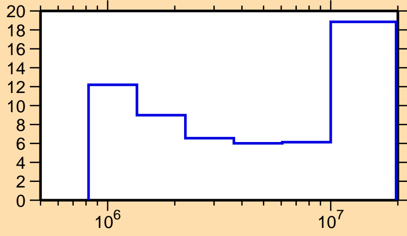
\Delta\sigma/\sigma vs. E for ^{173}\text{Yb}(n,\text{inel.})
