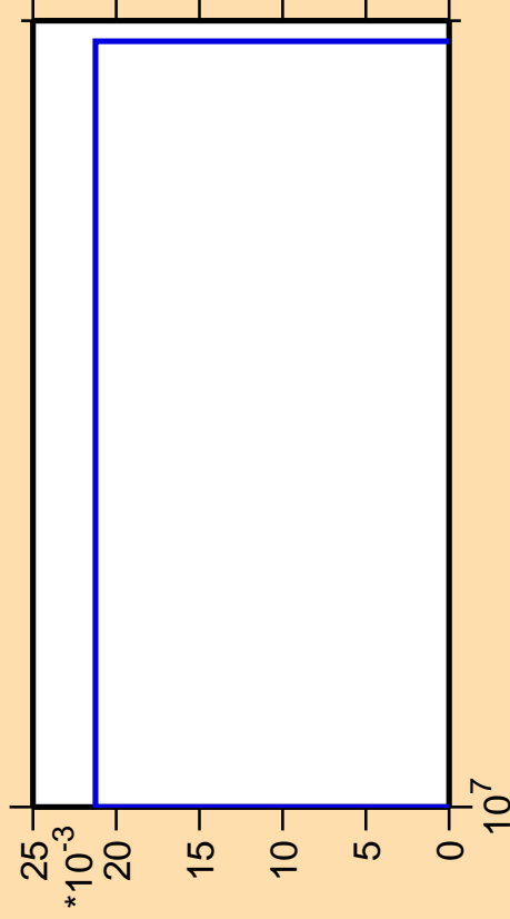
\Delta\sigma/\sigma vs. E for ^{173}\text{Yb}(n,p\alpha)
