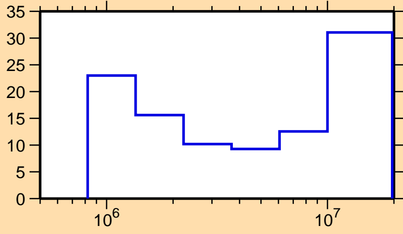
\Delta\sigma/\sigma vs. E for ^{173}\text{Yb}(n,n\text{cont.})
