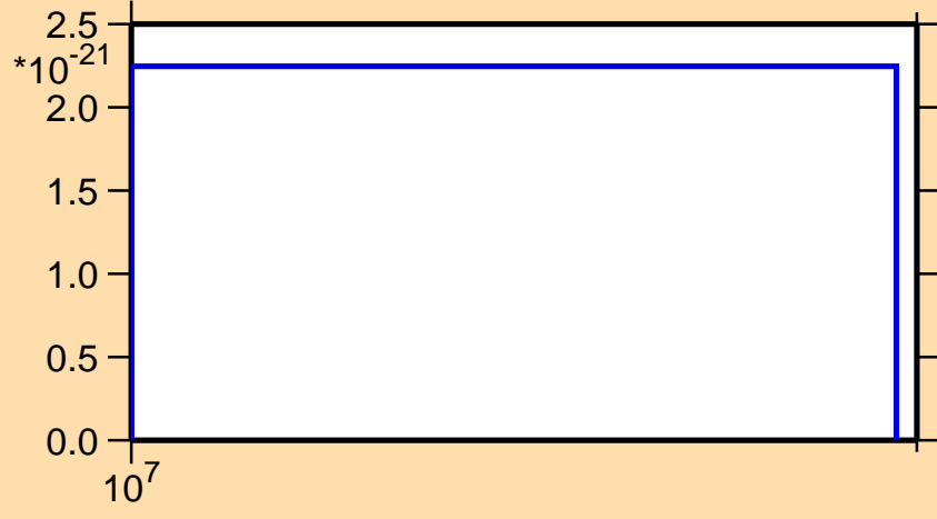
\sigma vs. E for ^{173}\text{Yb} (mt 11)
