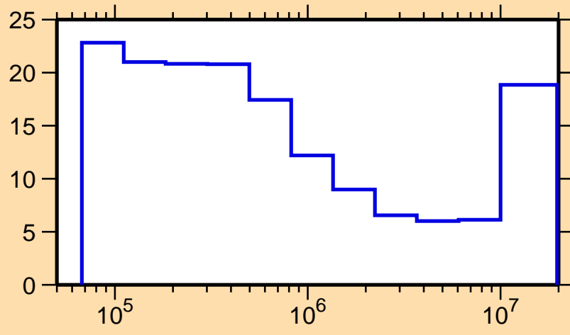
\Delta\sigma/\sigma vs. E for ^{173}\text{Yb}(n, \text{inel.})
