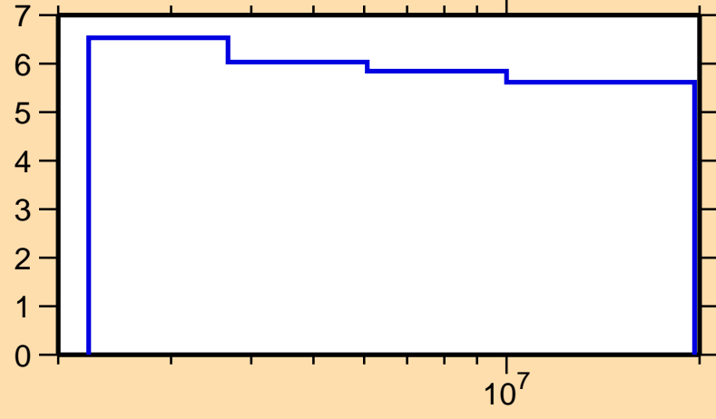
\Delta\sigma/\sigma vs. E for ^{173}\text{Yb}(n,\text{nonel.})
