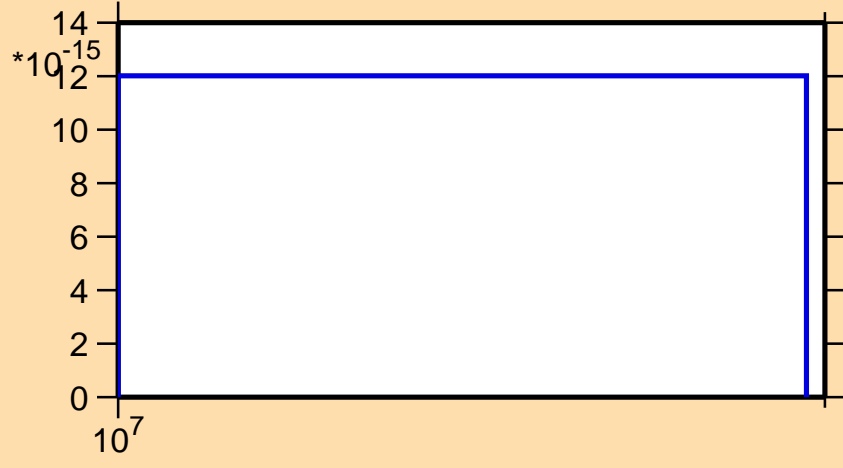
\sigma vs. E for ^{173}\text{Yb}(n,p\alpha)
