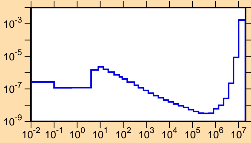
\sigma vs. E for ^{173}\text{Yb}(n,\alpha)
