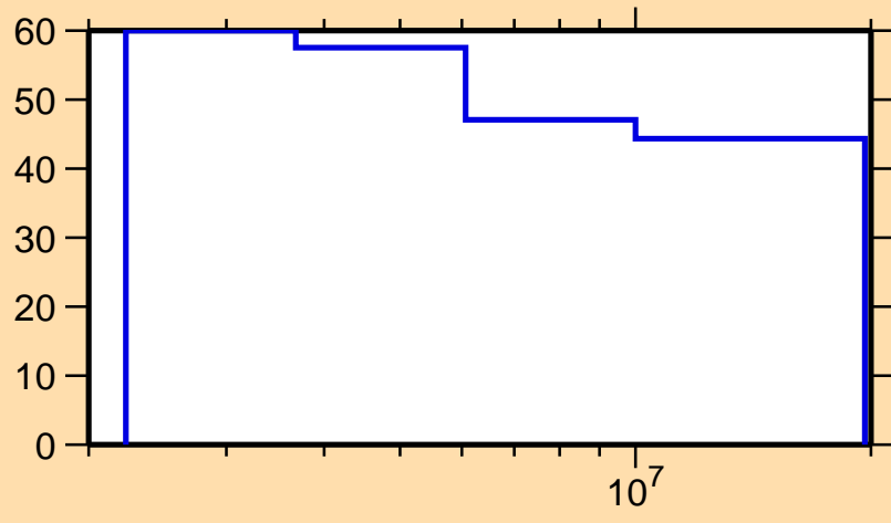
\Delta\sigma/\sigma vs. E for ^{173}\text{Yb}(n,p)
