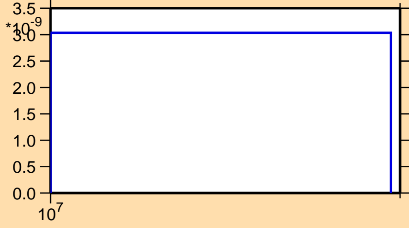
\sigma vs. E for ^{173}\text{Yb}(n,2np)
