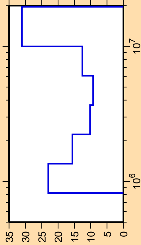
\Delta\sigma/\sigma vs. E for ^{173}\text{Yb}(n,n\text{cont.})
