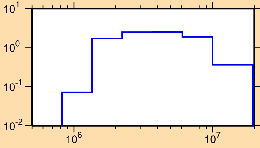
\sigma vs. E for ^{173}\text{Yb}(n,n\text{cont.})
