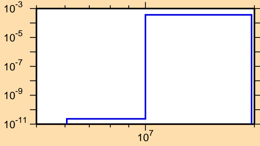
\sigma vs. E for ^{173}\text{Yb}(n,d)
