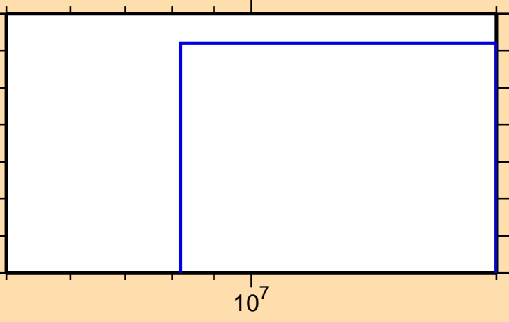
\sigma vs. E for ^{173}\text{Yb}(n,2n\alpha)
