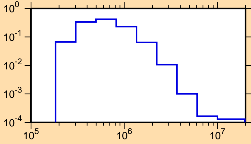
\sigma vs. E for ^{175}\text{Yb}(n,n_2)
