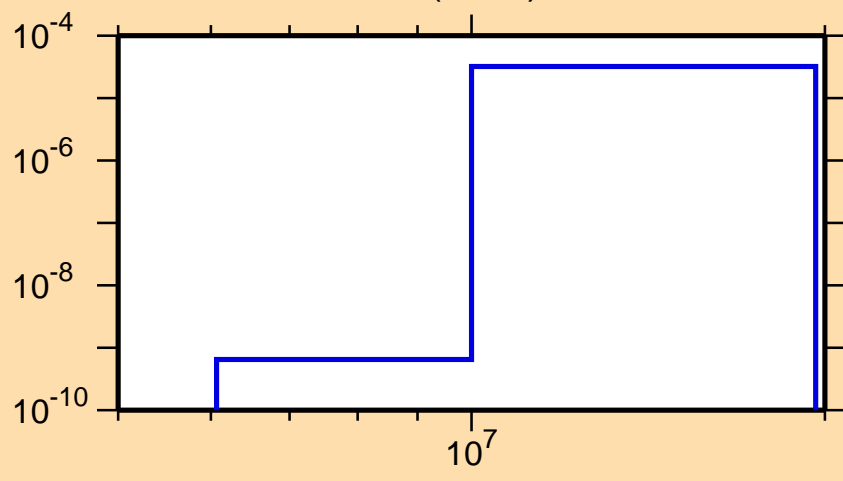
\sigma vs. E for ^{175}\text{Yb}(n,n\alpha)
