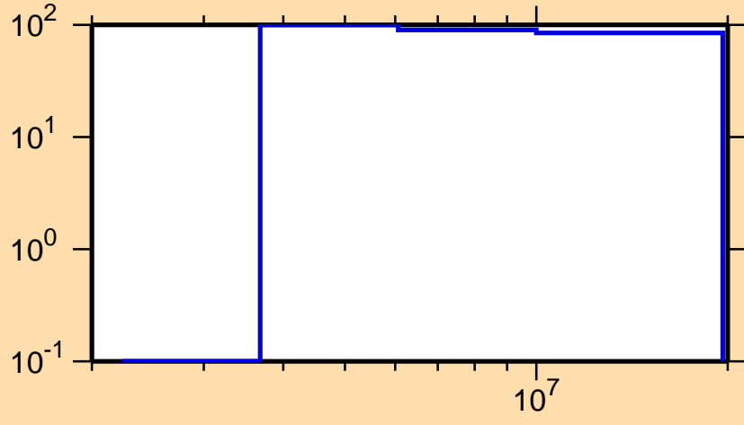
\Delta\sigma/\sigma vs. E for ^{175}\text{Yb}(n,p)
