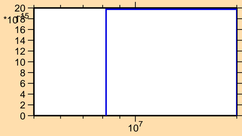
\sigma vs. E for ^{175}\text{Yb}(n,\text{He}3)
