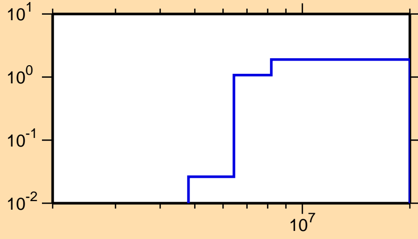
\sigma vs. E for ^{175}\text{Yb}(n,2n)
