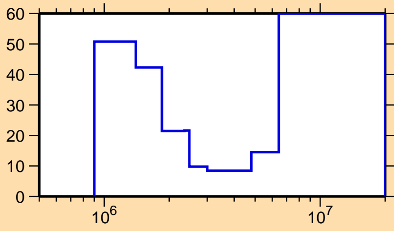
\Delta\sigma/\sigma vs. E for ^{175}\text{Yb}(n,n\text{cont.})
