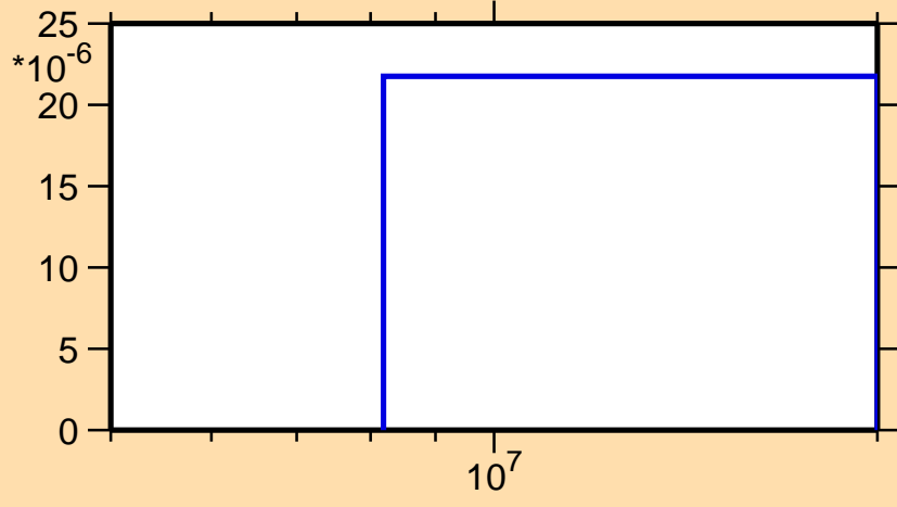
\sigma vs. E for ^{175}\text{Yb}(n,t)
