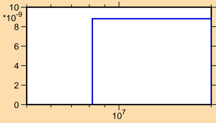
\sigma vs. E for ^{175}\text{Yb}(n,2n\alpha)
