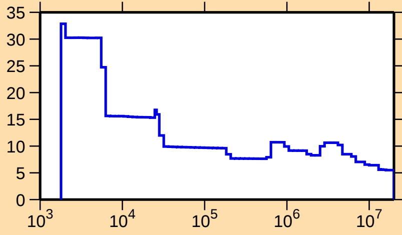
\Delta\sigma/\sigma vs. E for ^{176}\text{Yb}(n,\text{nonel.})
