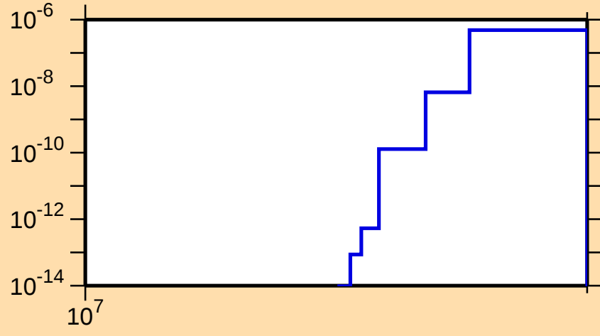
\sigma vs. E for ^{176}\text{Yb}(n,nt)
