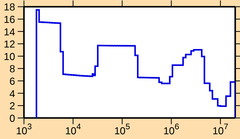
\Delta\sigma/\sigma vs. E for ^{176}\text{Yb}(n,\text{tot.})
