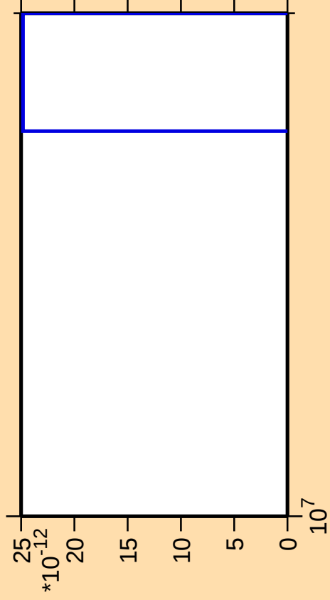
\Delta\sigma/\sigma vs. E for ^{176}\text{Yb} (mt 42)
