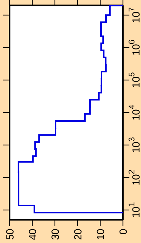
\Delta\sigma/\sigma vs. E for ^{176}\text{Yb}(n,\text{nonel.})
