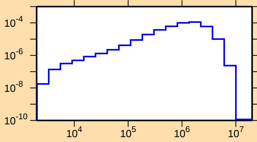
\sigma vs. E for ^{176}\text{Yb}(n,n_1)
