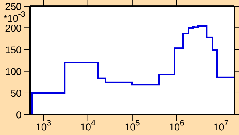
\sigma vs. E for ^{176}\text{Yb}(n,n_3)
