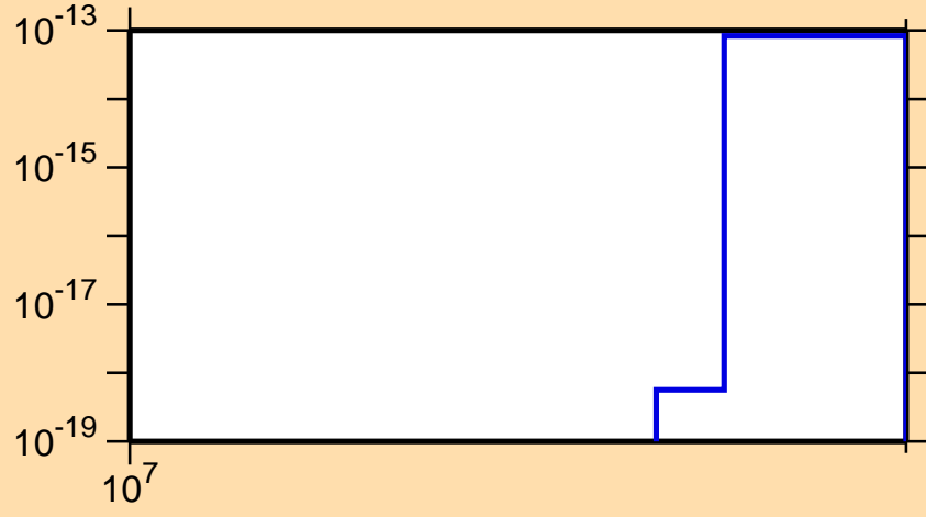
\sigma vs. E for ^{177}\text{Yb}(n,3n\alpha)
