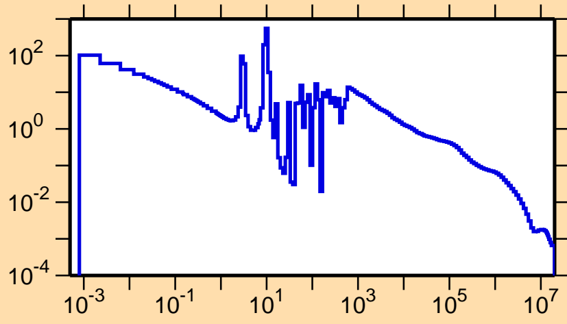
\sigma vs. E for ^{177}\text{Yb}(n,\gamma)
