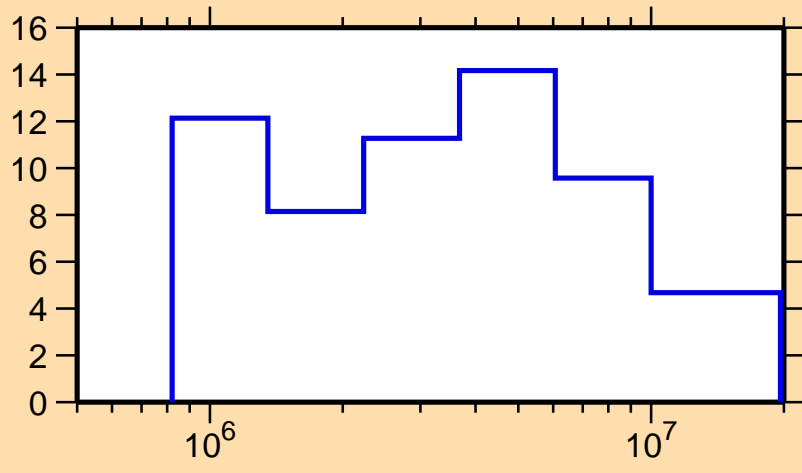
\Delta\sigma/\sigma vs. E for ^{177}\text{Yb}(n, tot.)
