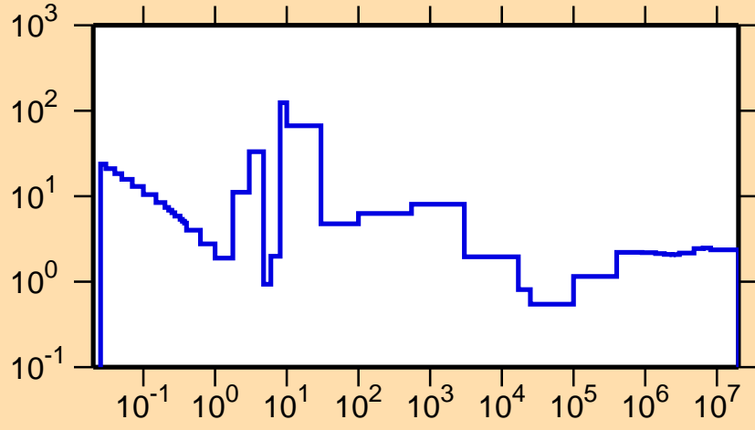
\sigma vs. E for ^{177}\text{Yb}(n,\text{nonel.})
