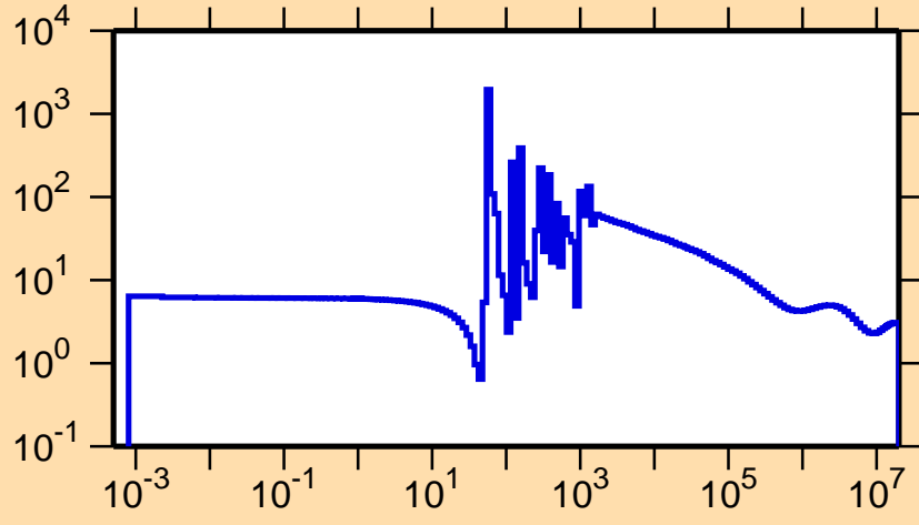
\sigma vs. E for ^{177}\text{Yb}(n,\text{el.})
