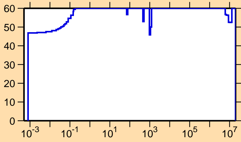
\Delta\sigma/\sigma vs. E for ^{177}\text{Yb}(n,\gamma)
