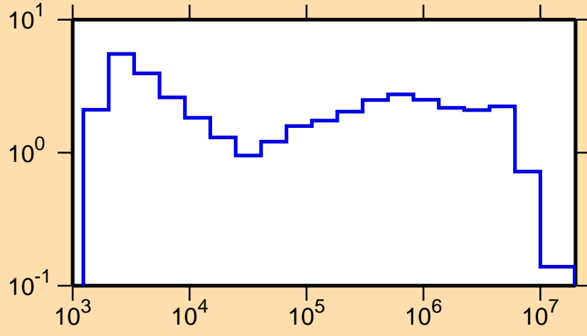
\sigma vs. E for ^{177}\text{Yb}(n,\text{inel.})
