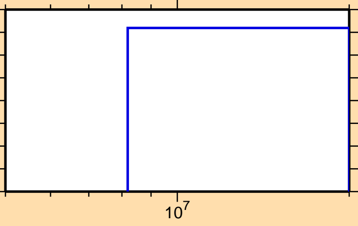
\sigma vs. E for ^{177}\text{Yb}(n,np)
