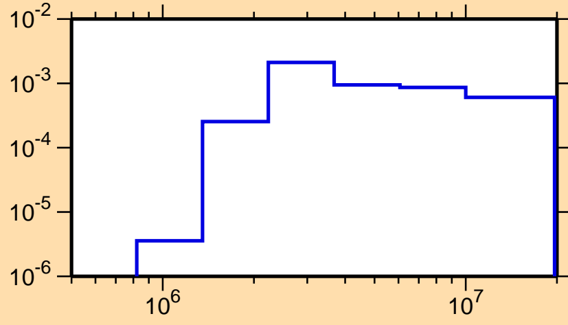
\sigma vs. E for ^{178}\text{Yb}(n,n_4)
