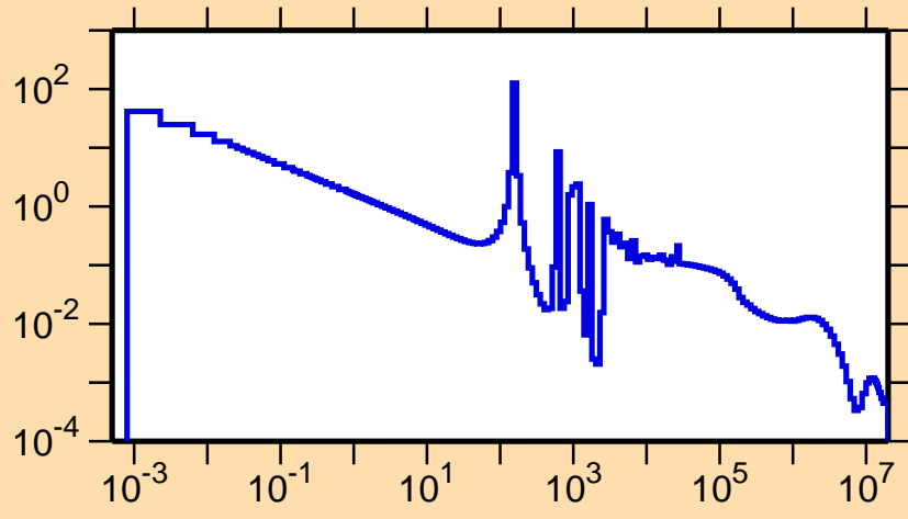
\sigma vs. E for ^{180}\text{Yb}(n,\gamma)
