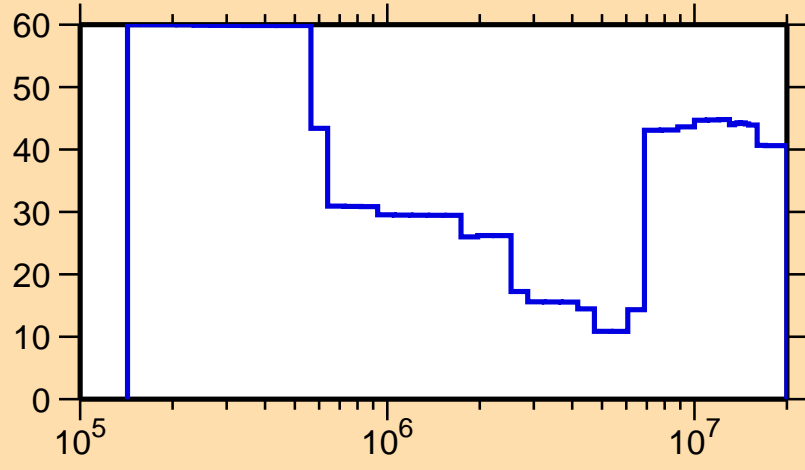
\Delta\sigma/\sigma vs. E for ^{180}\text{Yb}(n,n\text{cont.})
