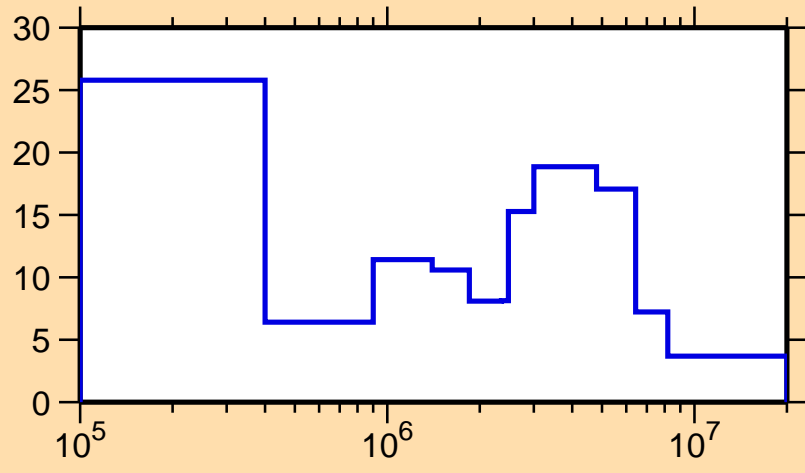
\Delta\sigma/\sigma vs. E for ^{180}\text{Yb}(n, el.)
