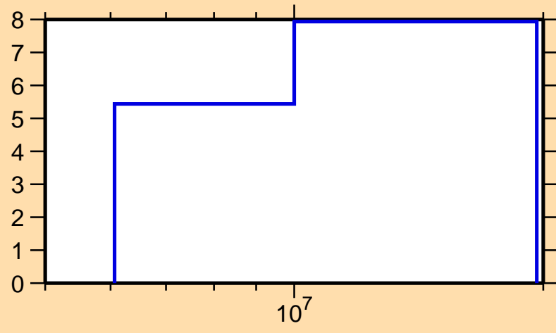
\Delta\sigma/\sigma vs. E for ^{181}\text{Yb}(n,el.)
