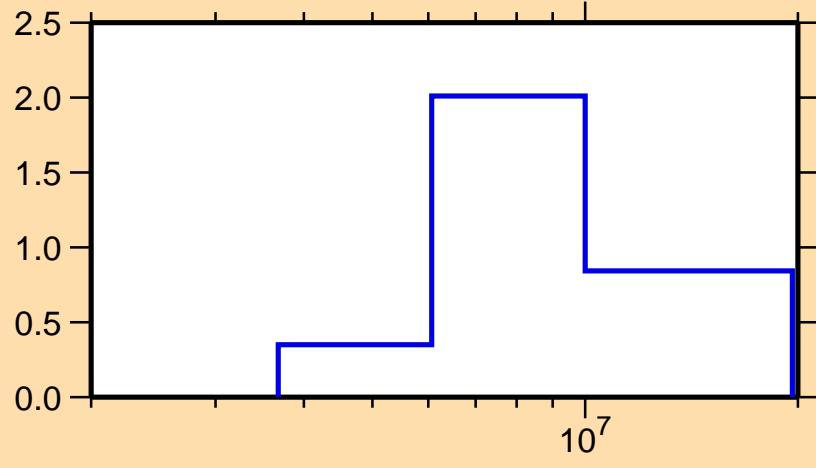
\sigma vs. E for ^{181}\text{Yb}(n,2n)
