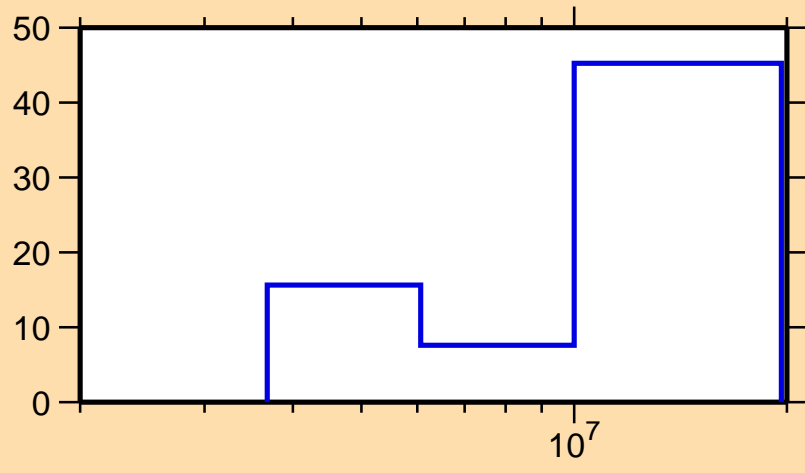
\Delta\sigma/\sigma vs. E for ^{181}\text{Yb}(n,2n)
