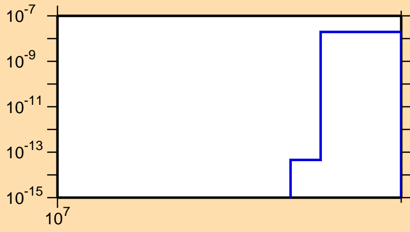
\sigma vs. E for ^{60}\text{Zn}(n,nd)
