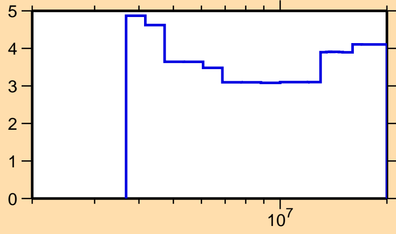
\Delta\sigma/\sigma vs. E for ^{60}\text{Zn}(n,n\text{onel.})
