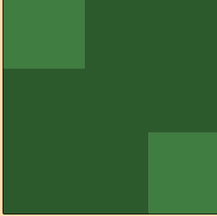
\sigma vs. E for ^{61}\text{Zn}(n,2n)
