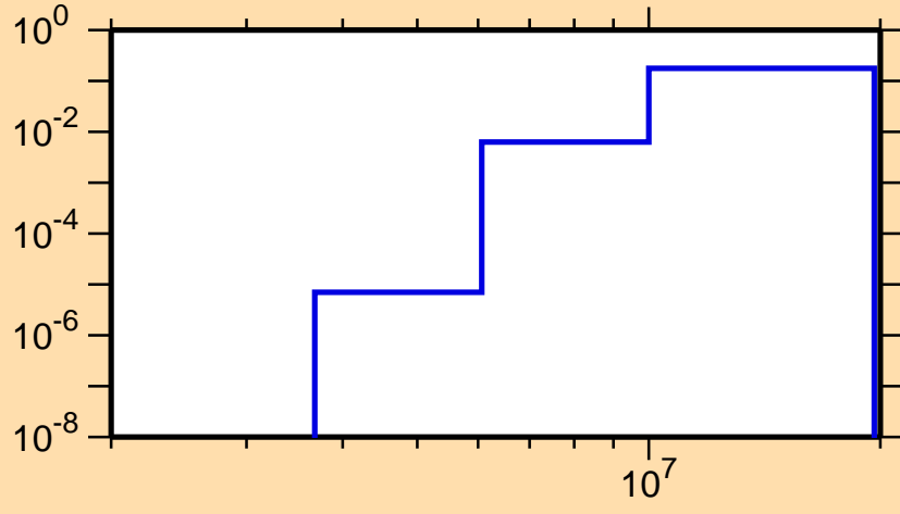
\sigma vs. E for ^{61}\text{Zn}(n,p\alpha)
