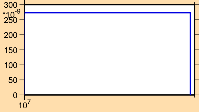
\sigma vs. E for ^{61}\text{Zn}(n,2np)
