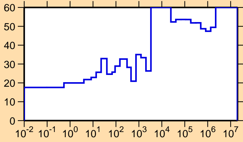
\Delta\sigma/\sigma vs. E for ^{61}\text{Zn}(n,\gamma)
