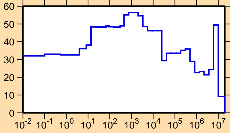
\Delta\sigma/\sigma vs. E for ^{61}\text{Zn}(n,p)
