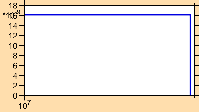
\sigma vs. E for ^{61}\text{Zn} (mt 45)
