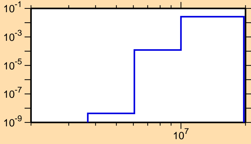
\sigma vs. E for ^{61}\text{Zn}(n,n\alpha)
