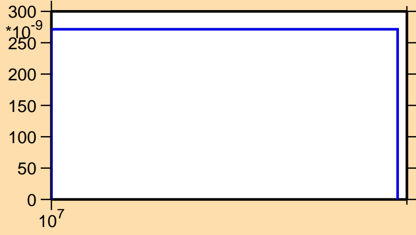
\sigma vs. E for ^{61}\text{Zn}(n,nd)
