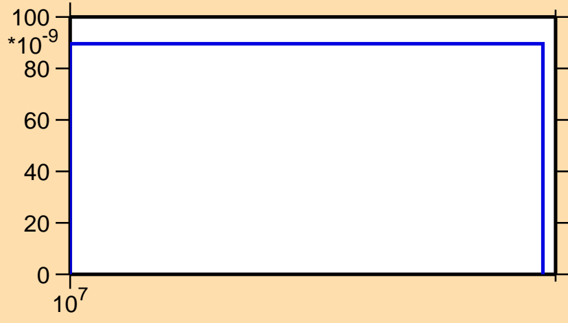
\sigma vs. E for ^{61}\text{Zn} (mt 34)
