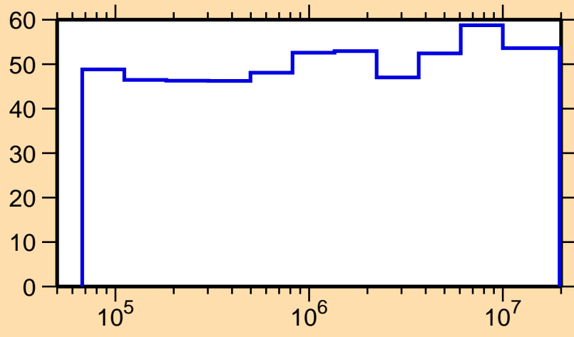
\Delta\sigma/\sigma vs. E for ^{61}\text{Zn}(n,n_1)
