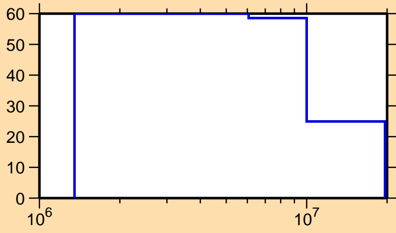
\Delta\sigma/\sigma vs. E for ^{61}\text{Zn}(n,n\text{cont.})
