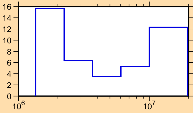
\Delta\sigma/\sigma vs. E for ^{61}\text{Zn}(n,\text{tot.})
