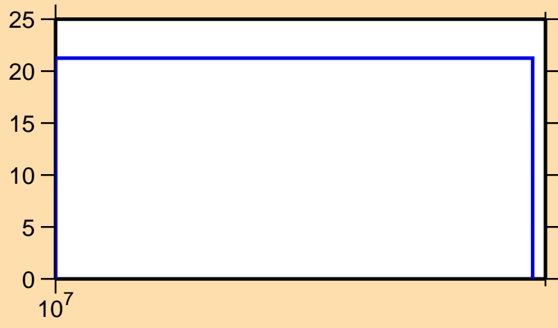
\Delta\sigma/\sigma vs. E for ^{61}\text{Zn}(n,\text{el.})
