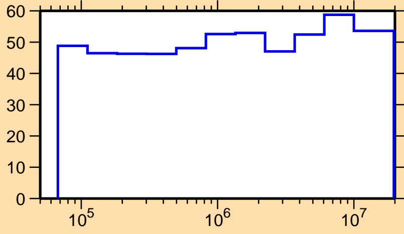
\Delta\sigma/\sigma vs. E for ^{61}\text{Zn}(n,n_1)
