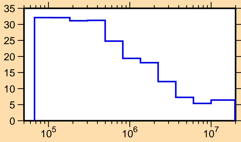
\Delta\sigma/\sigma vs. E for ^{61}\text{Zn}(n,\text{nonel.})
