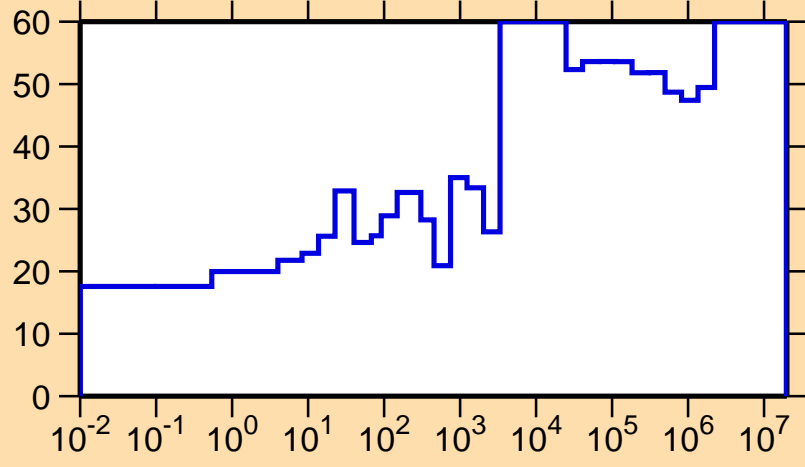
\Delta\sigma/\sigma vs. E for ^{61}\text{Zn}(n,\gamma)
