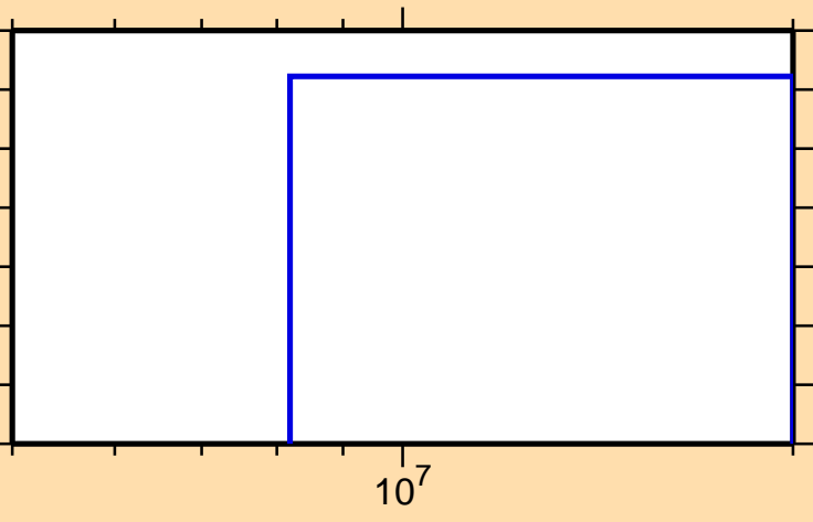
\sigma vs. E for ^{61}\text{Zn}(n,\text{pt})
