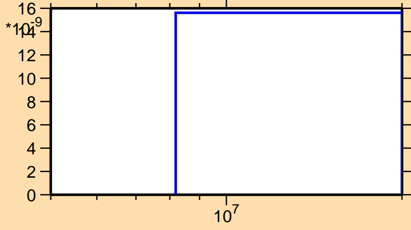
\sigma vs. E for ^{61}\text{Zn} (mt 45)
