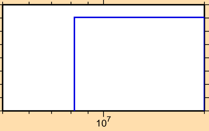
\sigma vs. E for ^{61}\text{Zn}(\text{mt117})
