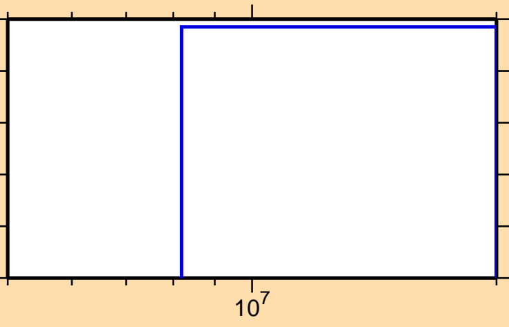
\sigma vs. E for ^{61}\text{Zn}(n,2n)
