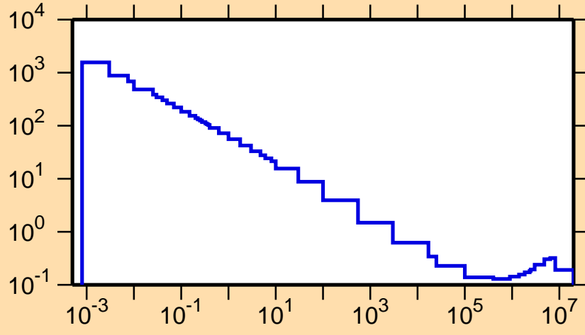
\sigma vs. E for ^{61}\text{Zn}(n,\alpha)
