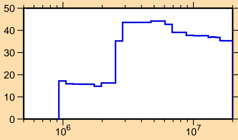
\Delta\sigma/\sigma vs. E for ^{62}\text{Zn}(n,n_1)
