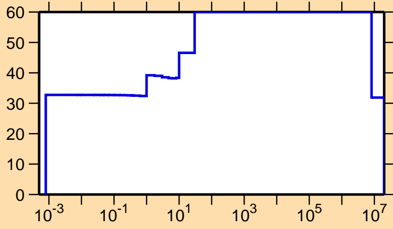
\Delta\sigma/\sigma vs. E for ^{62}\text{Zn}(n,\gamma)
