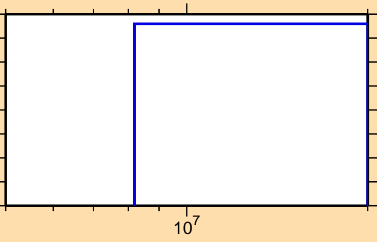
\sigma vs. E for ^{62}\text{Zn}(n,2np)
