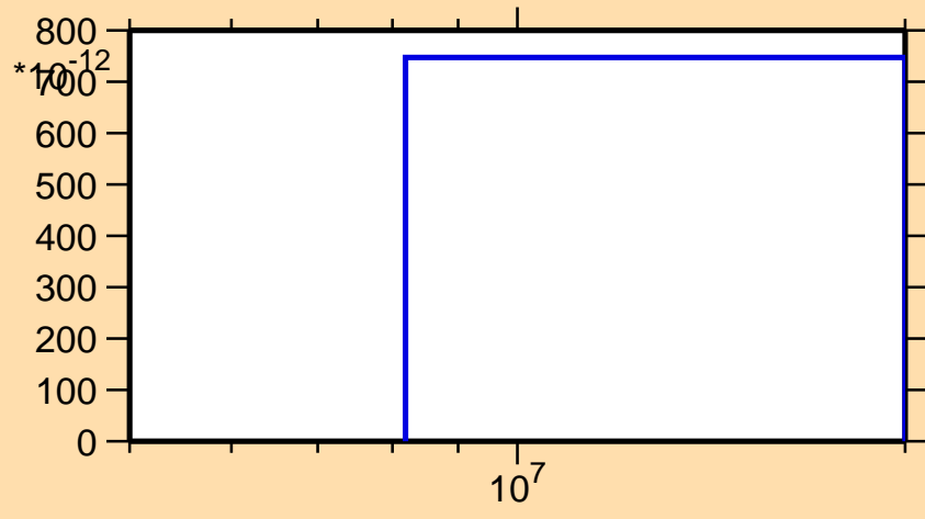
\sigma vs. E for ^{62}\text{Zn}(n,\text{nd})
