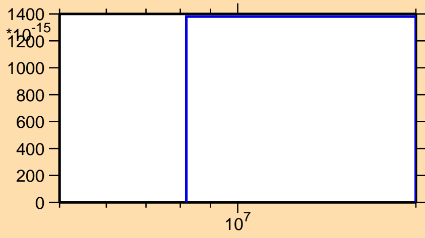
\sigma vs. E for ^{62}\text{Zn}(n,2n\alpha)
