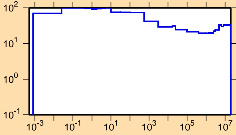
\Delta\sigma/\sigma vs. E for ^{62}\text{Zn}(n,p)
