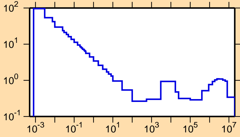
\sigma vs. E for ^{62}\text{Zn}(n,p)
