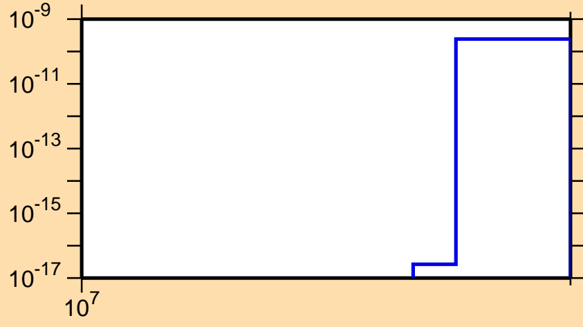
\sigma vs. E for ^{64}\text{Zn} (mt 45)
