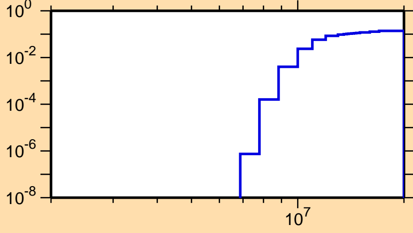
\sigma vs. E for ^{64}\text{Zn}(n,n\alpha)
