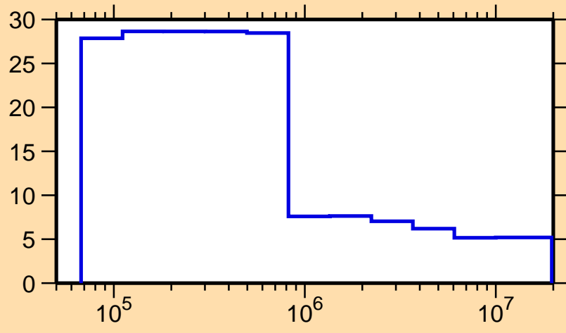
\Delta\sigma/\sigma vs. E for ^{64}\text{Zn}(n,\text{nonel.})
