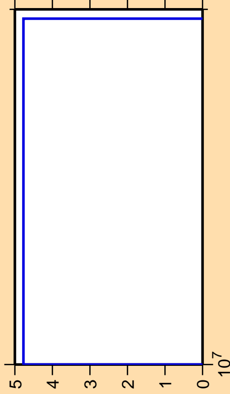
\Delta\sigma/\sigma vs. E for ^{64}\text{Zn}(n,2np)
