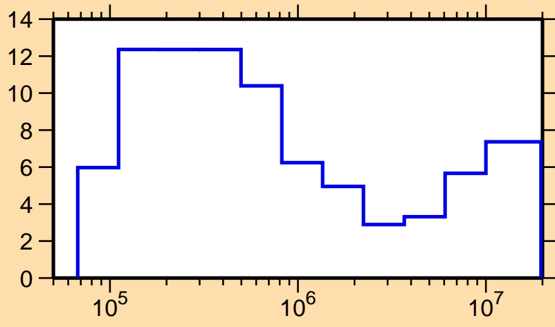
\Delta\sigma/\sigma vs. E for ^{64}\text{Zn}(n,\text{tot.})
