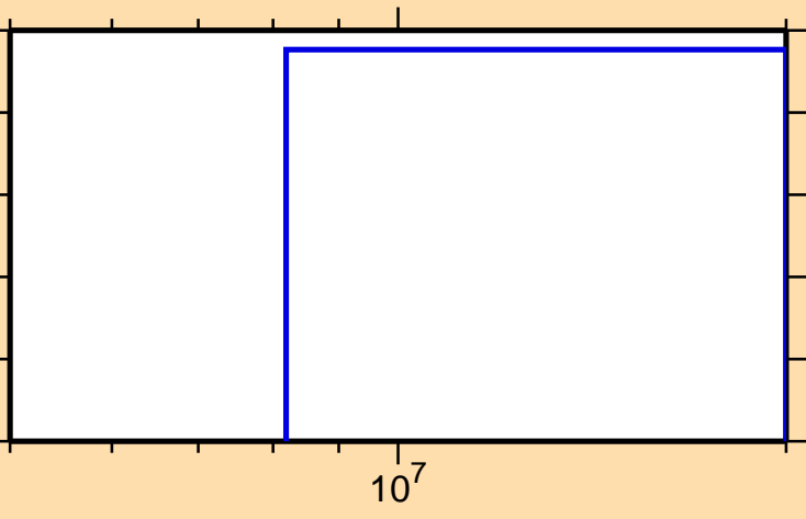
\sigma vs. E for ^{64}\text{Zn}(n,\text{He}3)
