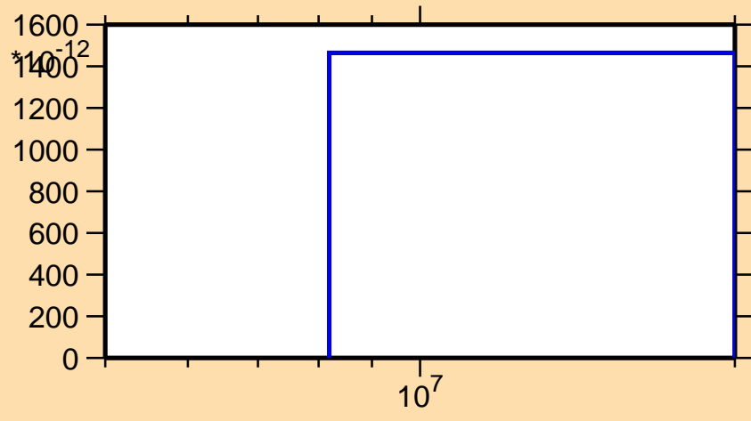
\sigma vs. E for ^{64}\text{Zn}(n,\text{nd})
