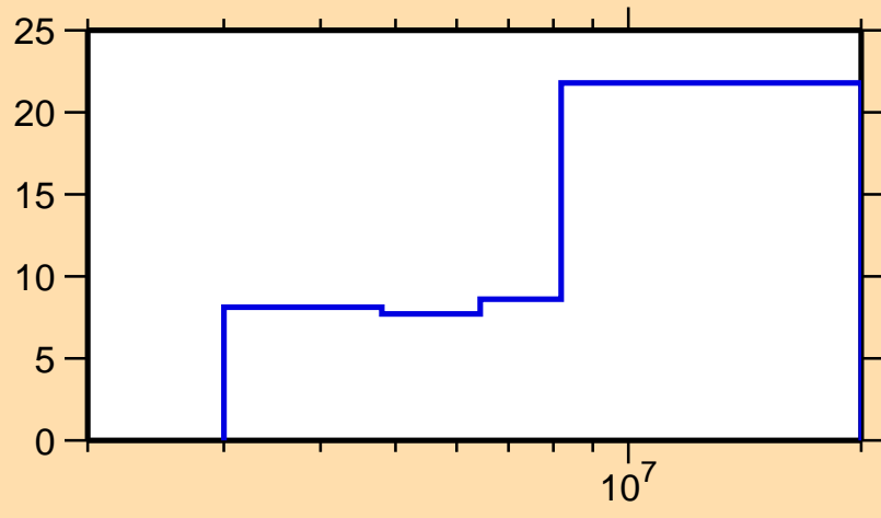
\Delta\sigma/\sigma vs. E for ^{64}\text{Zn}(n,ncont.)
