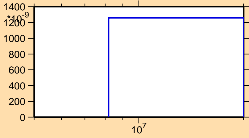
\sigma vs. E for ^{64}\text{Zn}(n,\text{pd})
