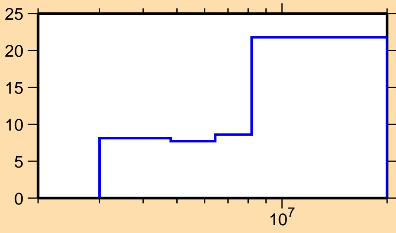
\Delta\sigma/\sigma vs. E for ^{64}\text{Zn}(n,n\text{cont.})
