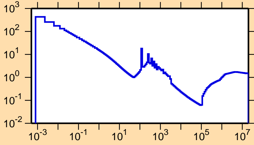
\sigma vs. E for ^{65}\text{Zn}(n,\text{nonel.})
