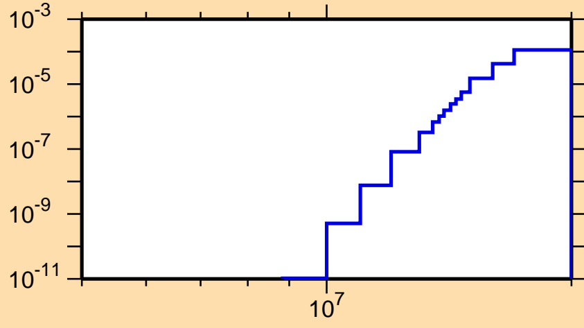
\sigma vs. E for ^{65}\text{Zn}(n,p\alpha)
