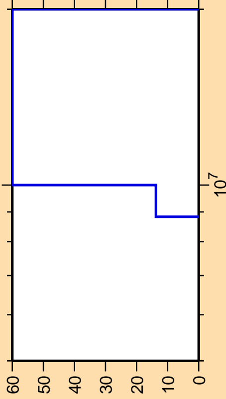
\Delta\sigma/\sigma vs. E for ^{65}\text{Zn}(n,p\alpha)
