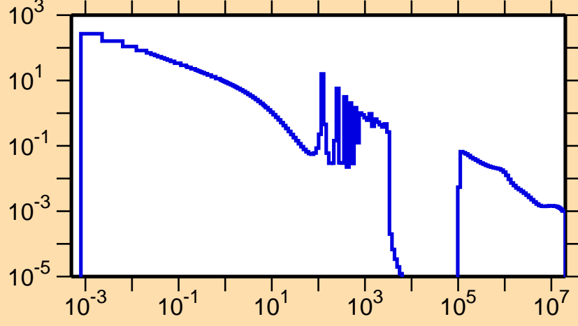
\sigma vs. E for ^{65}\text{Zn}(n,\gamma)
