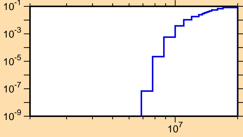
\sigma vs. E for ^{65}\text{Zn}(n,n\alpha)
