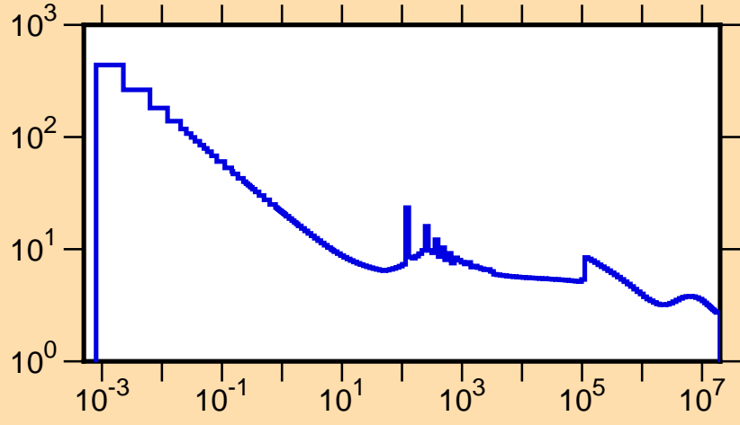
\sigma vs. E for ^{65}\text{Zn}(n,\text{tot.})
