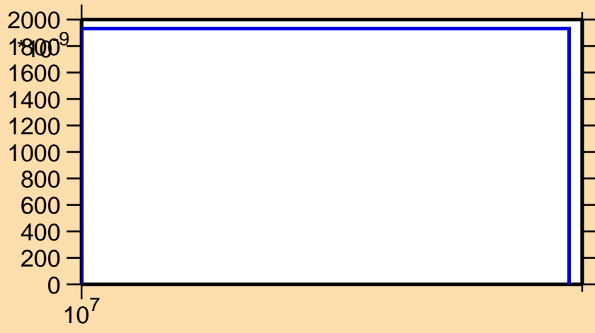
\sigma vs. E for ^{65}\text{Zn}(n,2n\alpha)
