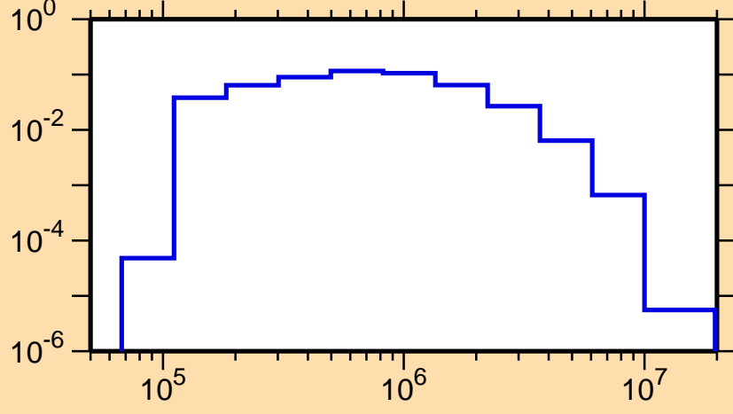
\sigma vs. E for ^{65}\text{Zn}(n,n_1)
