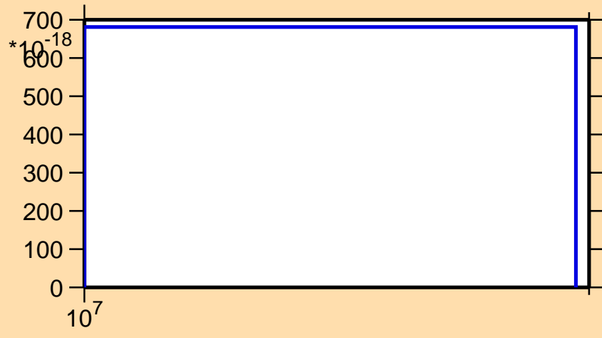
\sigma vs. E for ^{65}\text{Zn} (mt 45)
