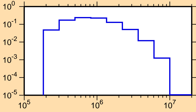
\sigma vs. E for ^{65}\text{Zn}(n,n_3)
