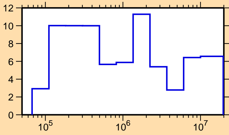
\Delta\sigma/\sigma vs. E for ^{65}\text{Zn}(n,\text{tot.})
