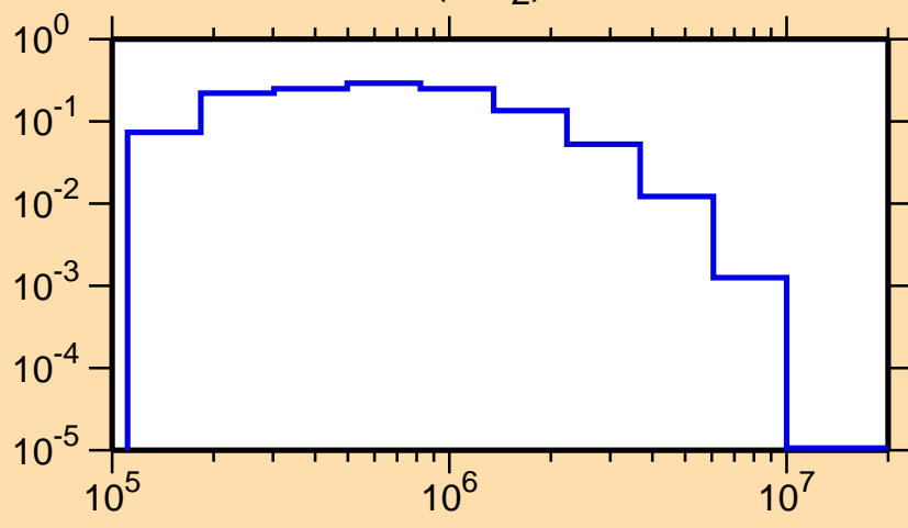
\sigma vs. E for ^{65}\text{Zn}(n,n_2)
