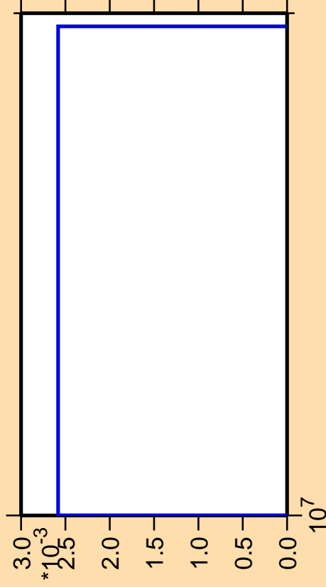
\Delta\sigma/\sigma vs. E for ^{65}\text{Zn} (mt 45)
