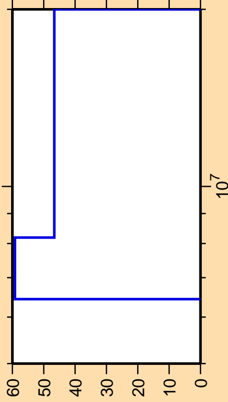
\Delta\sigma/\sigma vs. E for ^{65}\text{Zn}(n,p)
