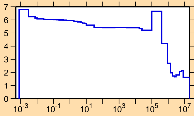
\sigma vs. E for ^{65}\text{Zn}(n,\text{el.})
