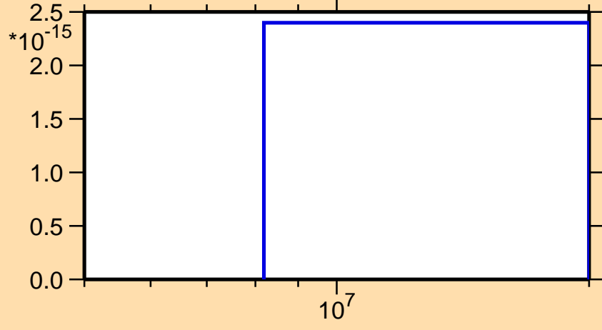
\sigma vs. E for ^{65}\text{Zn}(n,nt)
