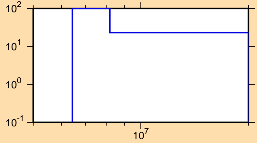
\Delta\sigma/\sigma vs. E for ^{65}\text{Zn}(n,2n)
