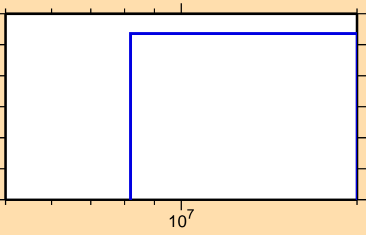
\sigma vs. E for ^{65}\text{Zn}(n,p\alpha)
