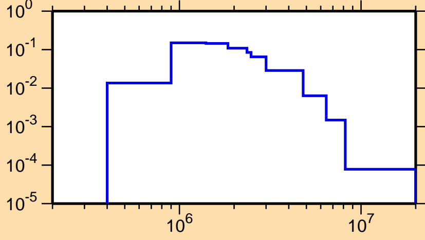
\sigma vs. E for ^{65}\text{Zn}(n,n_4)
