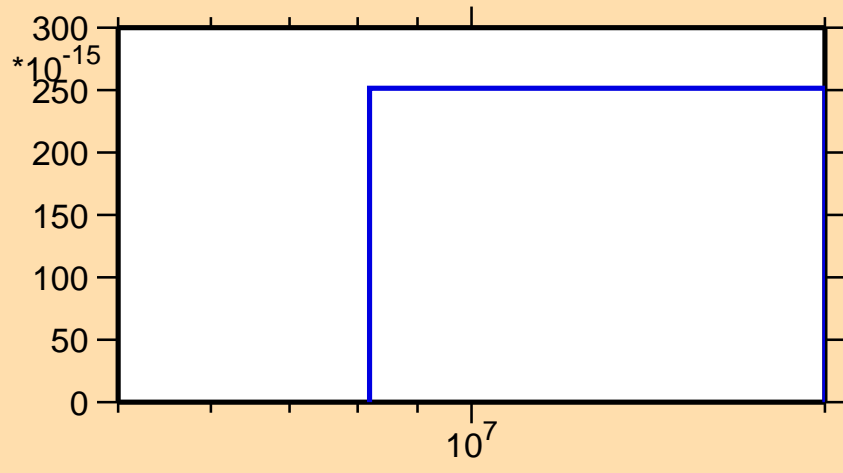
\sigma vs. E for ^{65}\text{Zn}(\text{mt117})
