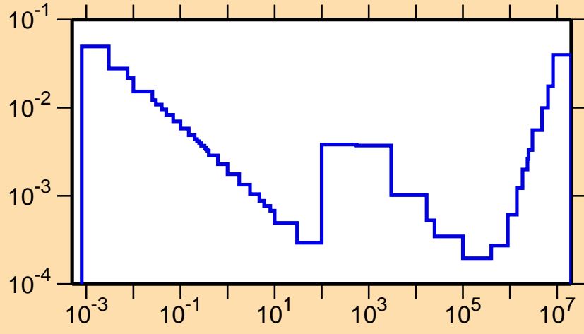
\sigma vs. E for ^{67}\text{Zn}(n,\alpha)
