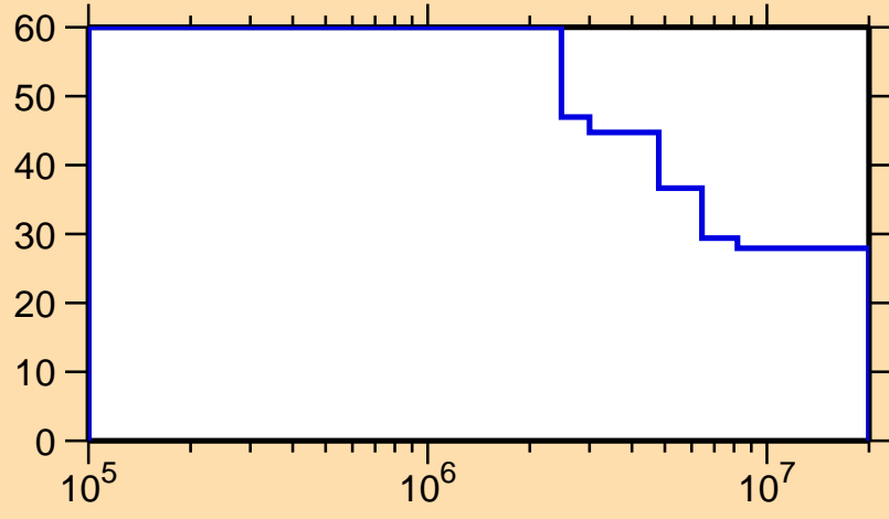
\Delta\sigma/\sigma vs. E for ^{67}\text{Zn}(n,p)
