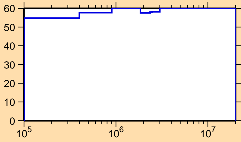
\Delta\sigma/\sigma vs. E for ^{67}\text{Zn}(n,\gamma)
