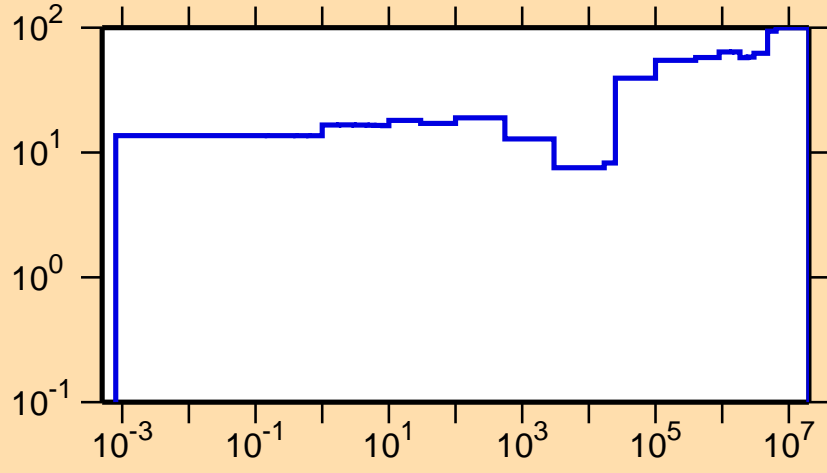
\Delta\sigma/\sigma vs. E for ^{67}\text{Zn}(n,\gamma)
