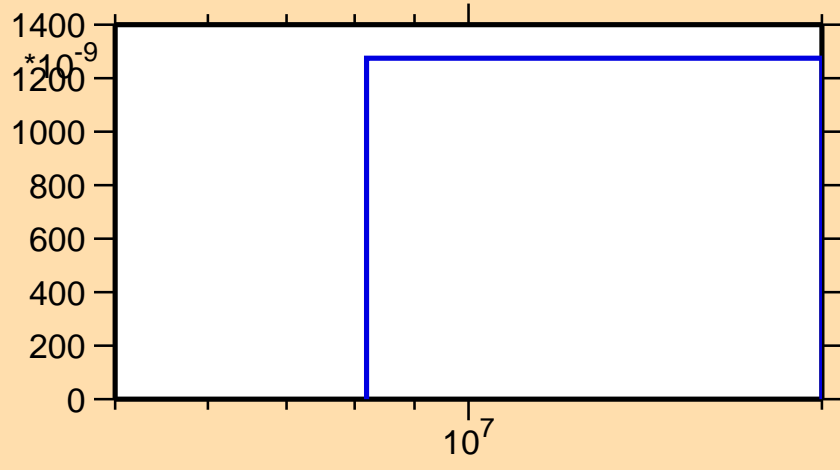
\sigma vs. E for ^{67}\text{Zn}(n,3n)
