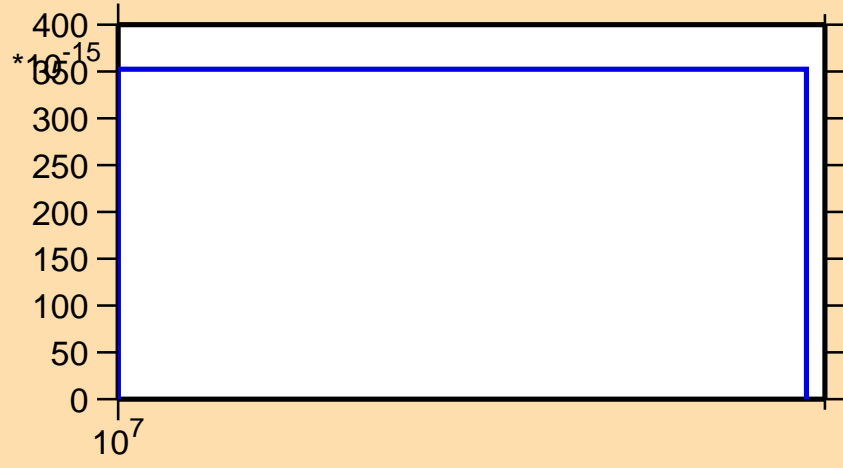
\sigma vs. E for ^{68}\text{Zn}(n,nt)
