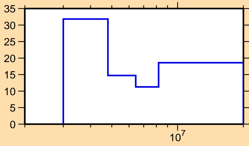
\Delta\sigma/\sigma vs. E for ^{68}\text{Zn}(n,ncont.)
