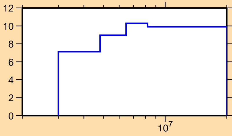
\Delta\sigma/\sigma vs. E for ^{68}\text{Zn}(n,el.)
