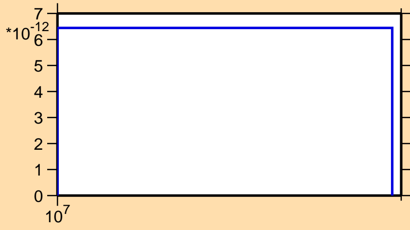
\sigma vs. E for ^{69}\text{Zn}(n,nt)
