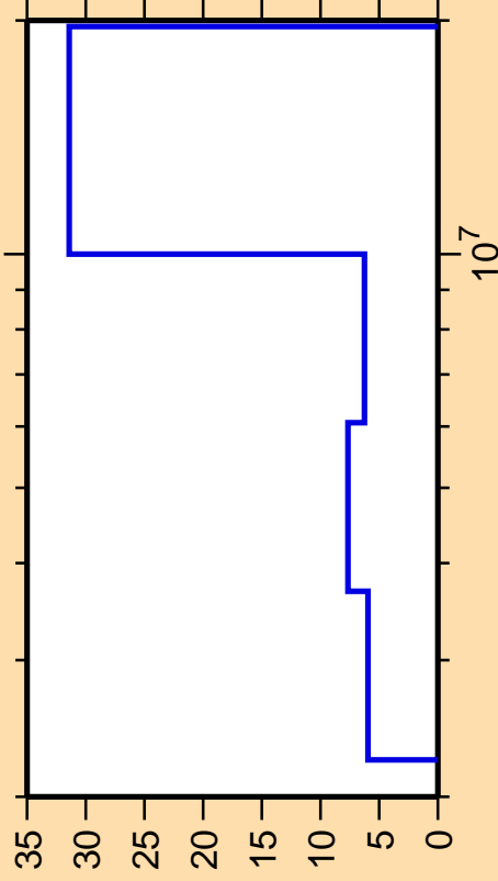
\Delta\sigma/\sigma vs. E for ^{69}\text{Zn}(n,n\text{cont.})
