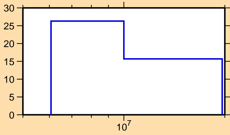
\Delta\sigma/\sigma vs. E for ^{69}\text{Zn}(n,2n)
