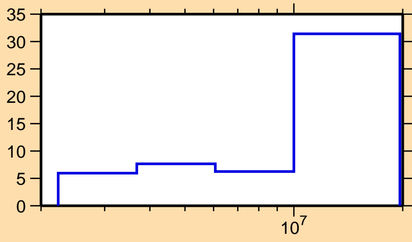
\Delta\sigma/\sigma vs. E for ^{69}\text{Zn}(n,n\text{cont.})
