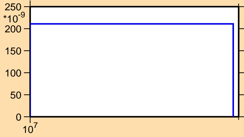
\sigma vs. E for ^{69}\text{Zn}(n,nd)
