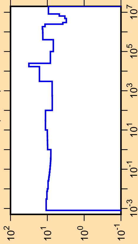
\Delta\sigma/\sigma vs. E for ^{69}\text{Zn}(n,\text{tot.})
