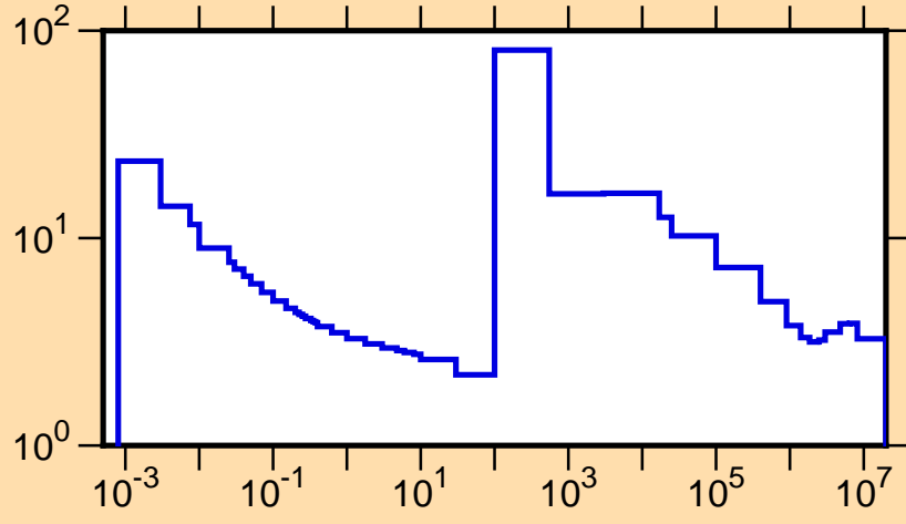
\sigma vs. E for ^{69}\text{Zn}(n,\text{tot.})
