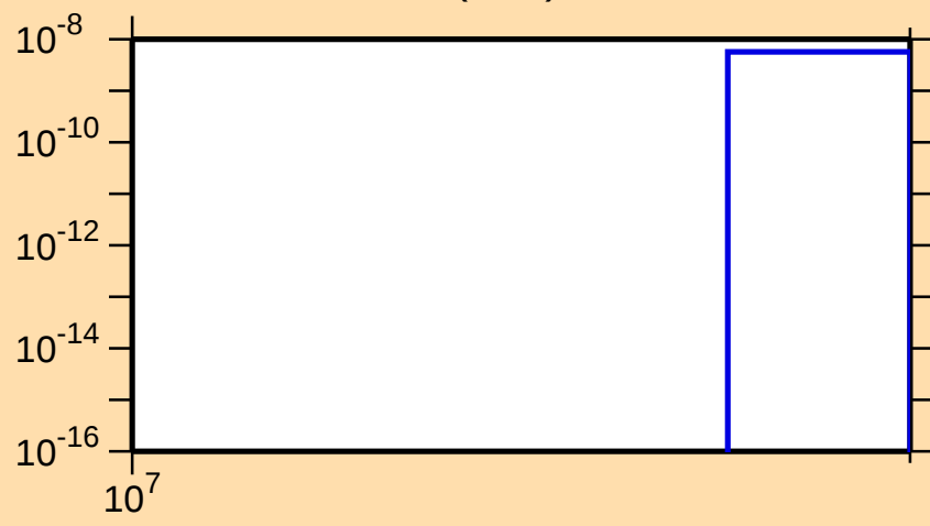
\sigma vs. E for ^{69}\text{Zn}(n,\text{nt})
