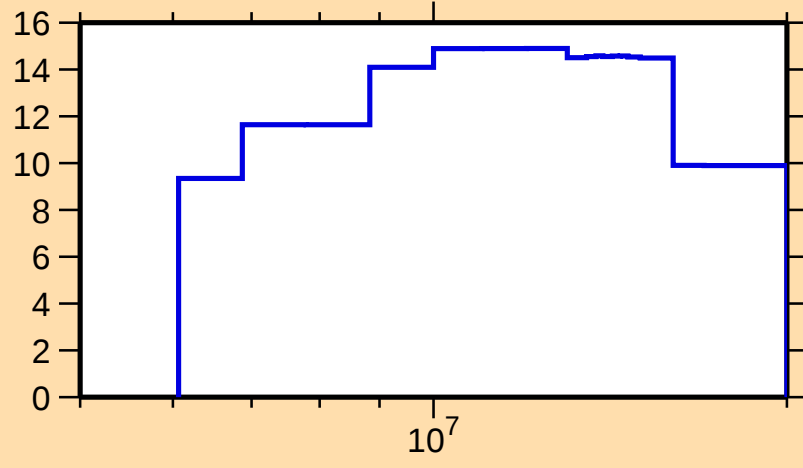
\Delta\sigma/\sigma vs. E for ^{69}\text{Zn}(n,\text{el.})
